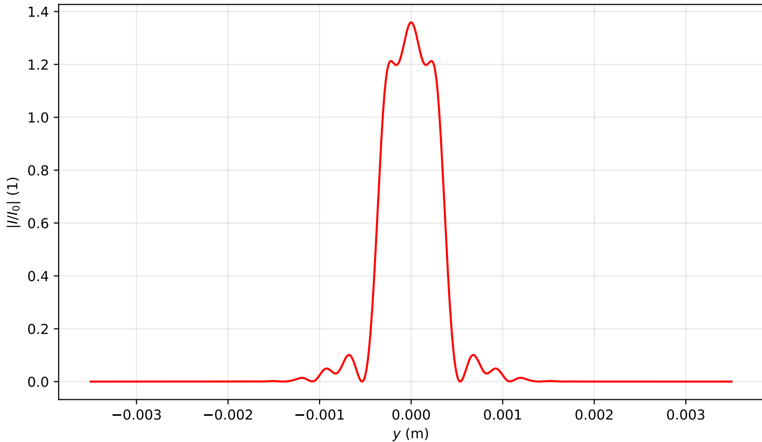
Intensity profile I(x=0, y, z=0.955)/I_0 , P_{in}=4.5P_{cr} , artificial time
